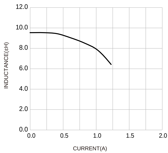
Inductance VS. Current Characteristics:
